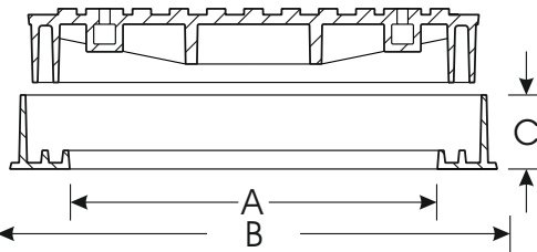
SECTIONAL VIEW OF COVER & FRAME
