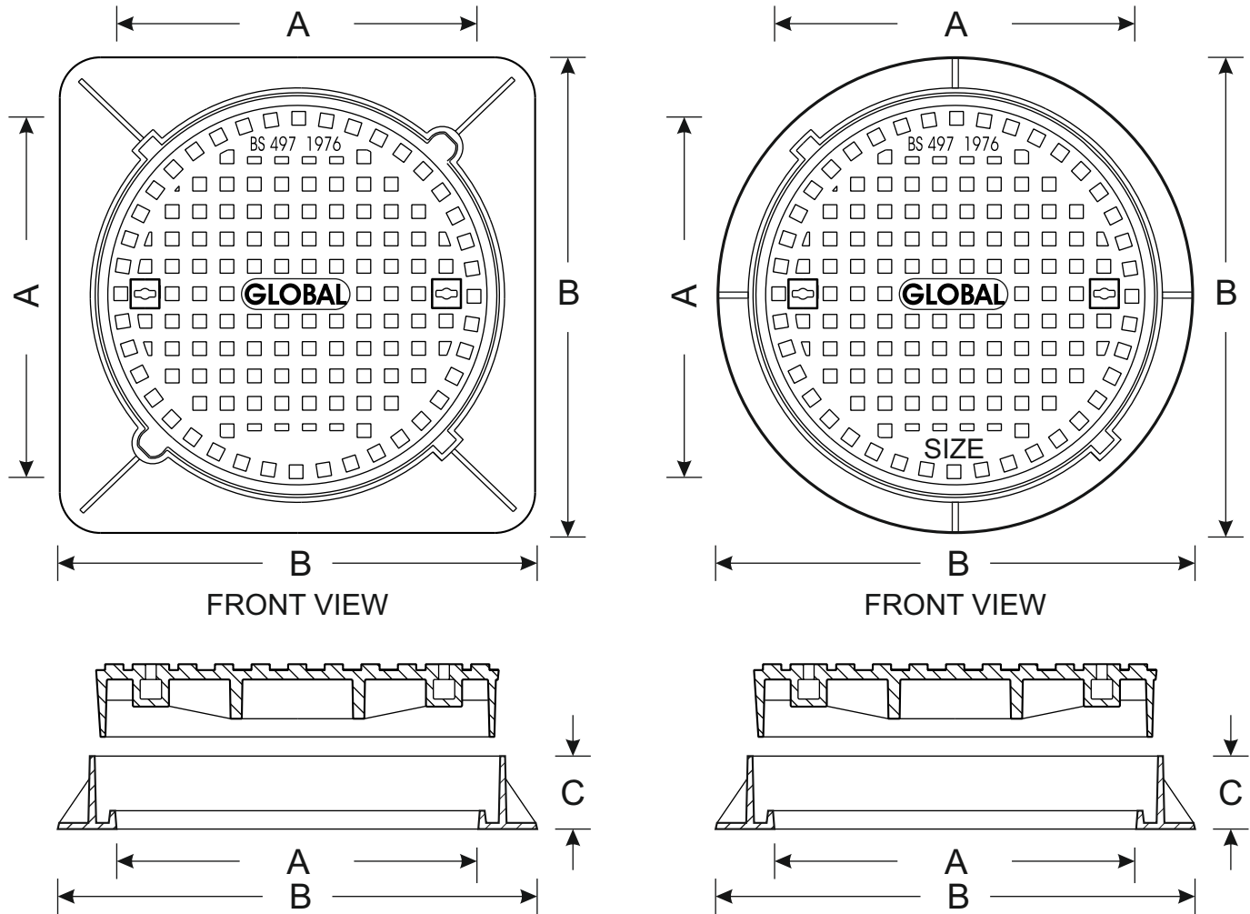
SECTIONAL VIEW OF COVER & FRAME
